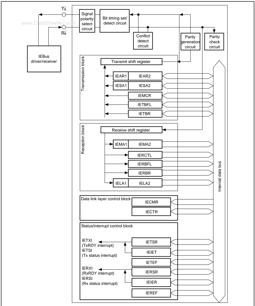
Figure 14.1 Block Diagram of IEB
