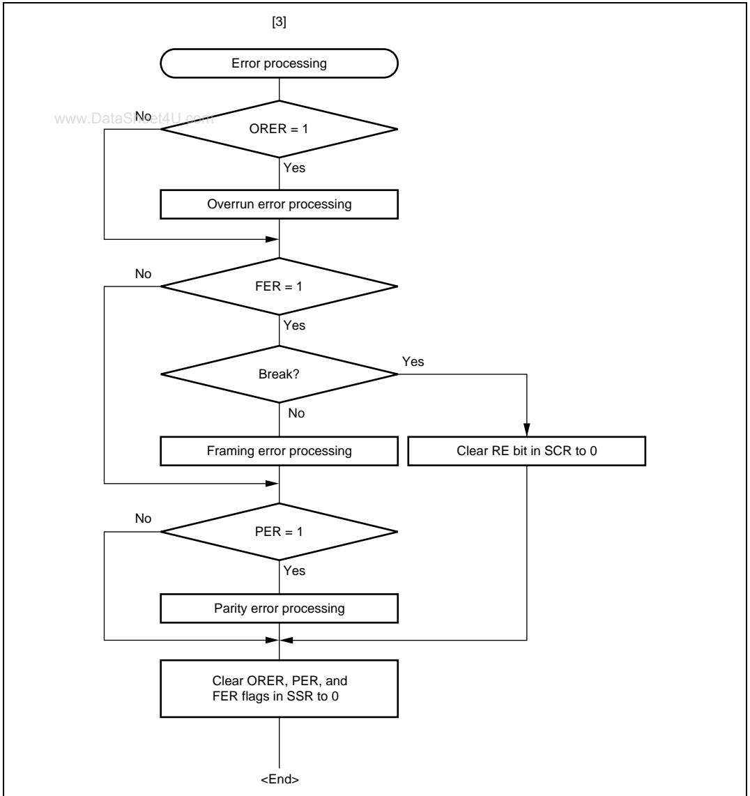
Figure 15.12 Sample Serial Reception Data Flowchart (2)
