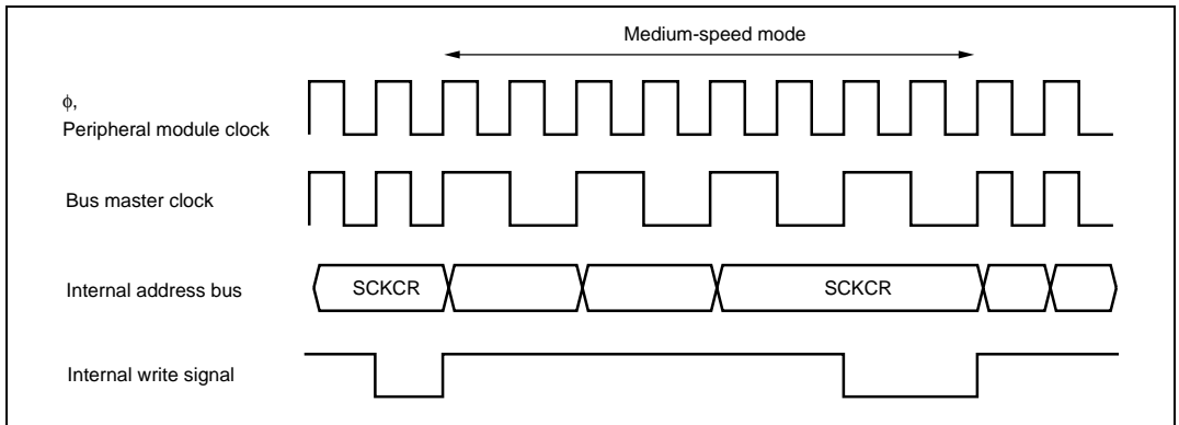
Figure 24.2 Medium-Speed Mode Transition and Clearance Timing
