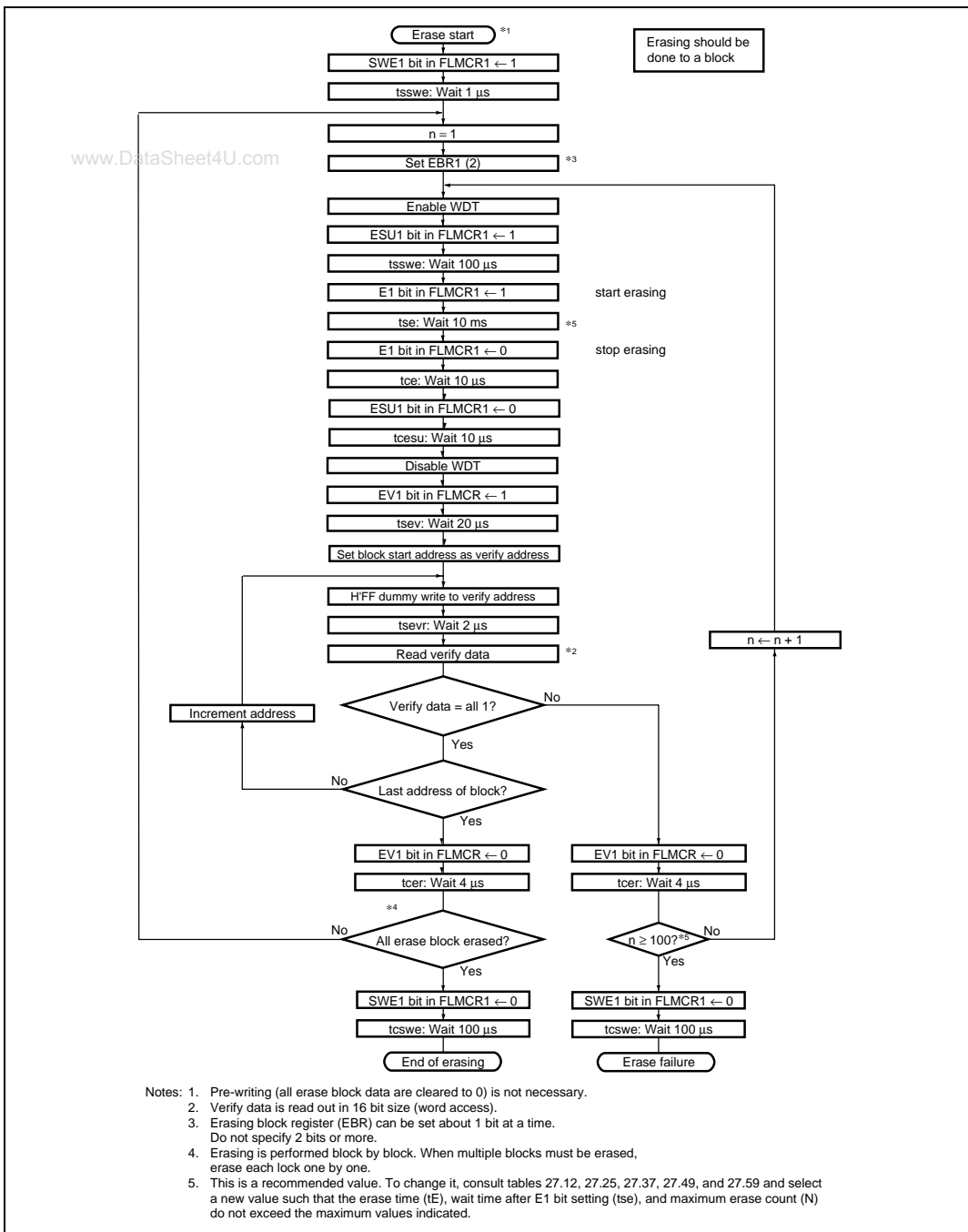
Figure 20.12 Erase/Erase-Verify Flowchart
