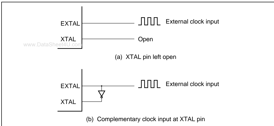
Figure 23.4 External Clock Input (Examples)
